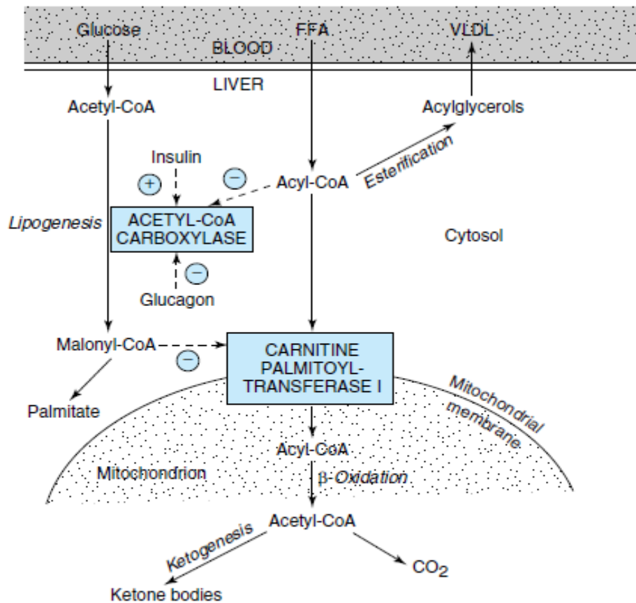
Figure 22-10. Regulation of long-chain fatty acid oxidation in the liver. (FFA, free fatty acids; VLDL, very low density lipoprotein.) Positive ( \oplus ) and negative ( \ominus ) regulatory effects are represented by broken arrows and substrate flow by solid arrows.
