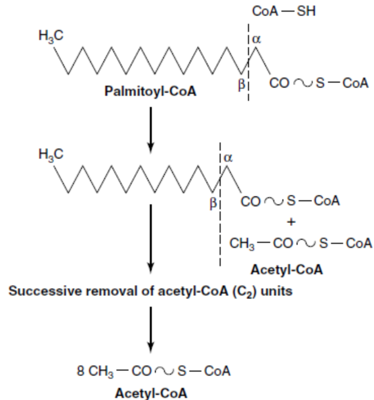
Figure 22-2. Overview of β-oxidation of fatty acids.
